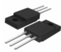
TYN16X-600CT,127 WeEn Semiconductors IC SCR 16A 600V TO-220F
