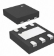
MIC5528-3.3YMX-T5 Microchip Technology IC REG LDO 3.3V 0.5A 6DFN
