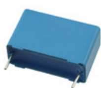
B32523Q8104J000 EPCOS CAP FILM 0.1UF 5% 630VDC RADIAL
