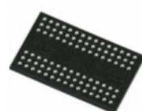
MT48H16M32LFB5-75 IT:C Micron Technology Inc. IC SDRAM 512MBIT 133MHZ 90VFBGA
