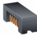
SRF3216A-261Y Bourns Inc. CMC 300MA 2LN 260OHM SMD AECQ200
