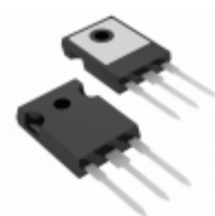
30CPF04 Electro-Films (EFI) / Vishay DIODE GEN PURP 400V 30A TO247AC
