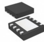
MCP4011T-202E/MC Microchip Technology IC DGTL POT 2.1K 1CH 8DFN
