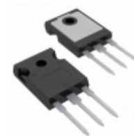
IRGP4266-EPBF Infineon Technologies IGBT 650V 140A 450W TO247AD
