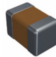
CDR31BP180BJZMAT Electro-Films (EFI) / Vishay CAP CER 18PF 100V 5% BP 0805
