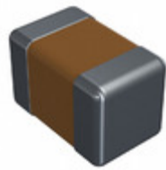
CDR31BP180BJZPAT Electro-Films (EFI) / Vishay CAP CER 18PF 100V 5% BP 0805
