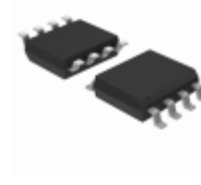
AT24C11N-10SU-2.7 Micrel / Microchip Technology IC EEPROM 1KBIT 1MHZ 8SOIC
