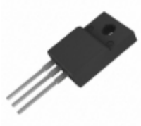
FQPF5N20L Fairchild/ON Semiconductor MOSFET N-CH 200V 3.5A TO-220F
