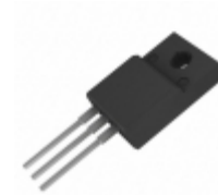
FQPF5N15 Fairchild/ON Semiconductor MOSFET N-CH 150V 4.2A TO-220F
