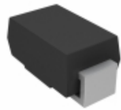
SML4744-E3/61 Vishay Semiconductor Diodes Division DIODE ZENER 15V 1W DO214AC
