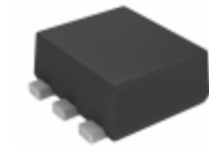
US6T7TR Rohm Semiconductor TRANS PNP 30V 1.5A TUMT6
