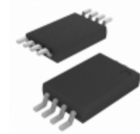
BR24G256FVT-3GE2 Rohm Semiconductor IC EEPROM 256KBIT 400MHZ 8TSSOP
