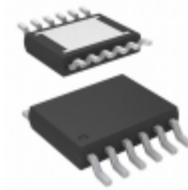
LTC3624HMSE-3.3#PBF ADI (Analog Devices, Inc.) IC REG BUCK 3.3V 2A SYNC 12MSOP
