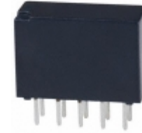
TN2-L2-H-6V Panasonic Electric Works RELAY GENERAL PURPOSE DPDT 1A 6V
