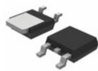
NCP1117DT20RKG ON Semiconductor IC REG LDO 2V 1A DPAK
