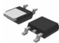
NCP1117DT25G ON Semiconductor IC REG LDO 2.5V 1A DPAK
