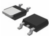
NCP1117DT18T5G ON Semiconductor IC REG LDO 1.8V 1A DPAK
