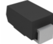
P4SMA20CA-E3/5A Vishay Semiconductor Diodes Division TVS DIODE 17.1VWM 27.7VC SMA
