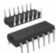
PIC16F18324-E/P Microchip Technology IC MCU 8BIT 7KB FLASH 14DIP
