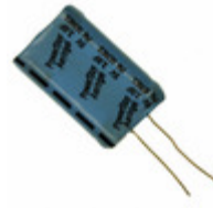
PM-5R0V305-R Eaton CAP 3F -20% +80% 5V T/H
