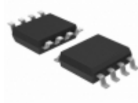
BR24G256F-3AGTE2 Rohm Semiconductor IC EEPROM 256KBIT 1MHZ 8SOP
