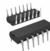
DM74AS20N Fairchild/ON Semiconductor IC GATE NAND 2CH 4-INP 14-DIP
