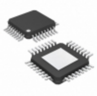
PL138-18FI Microchip Technology IC CLK BUFFER 2:10 700MHZ 32LQFP
