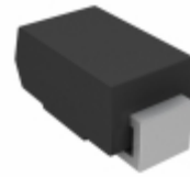
SMAJ78A-E3/5A Vishay Semiconductor Diodes Division TVS DIODE 78VWM 126VC SMA
