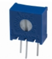
3386X-EY5-502LF Bourns, Inc. TRIMMER 5K OHM 0.5W PC PIN SIDE
