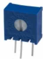
3386X-EY5-503LF Bourns, Inc. TRIMMER 50K OHM 0.5W PC PIN SIDE
