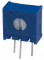
3386X-EY5-504 Bourns, Inc. TRIMMER 500KOHM 0.5W PC PIN SIDE
