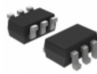
NCS199A1SQT2G ON Semiconductor IC CURRENT SENS AMP SC-88-6
