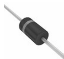
ICTE-022G ON Semiconductor TVS DIODE 22VWM 37.5VC AXIAL
