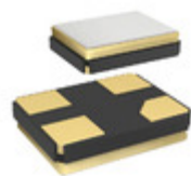
FA-20H 26.0000ML81Z-AC3 EPSON CRYSTAL 26.0000MHZ 9PF SMD
