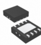
ISL80031AFRZ-T7A Intersil IC REG BUCK ADJ 3A SYNC 8DFN
