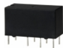
G5V-2-H1 DC48 Omron Electronics Inc-EMC Div RELAY GEN PURPOSE DPDT 1A 48V
