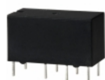
G5V-2-H1 DC12 Omron Electronics Inc-EMC Div RELAY GEN PURPOSE DPDT 1A 12V
