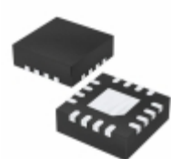
MCP4641T-502E/ML Microchip Technology IC DGTL POT 5K 129TAPS 16-QFN
