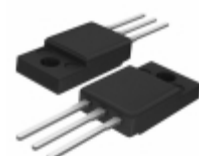
ACTT10X-800EQ WeEn Semiconductors TRIAC SENS GATE 800V 10A TO220FP
