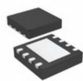
MCP1754ST-1802E/MC Microchip Technology IC REG LDO 1.8V 0.15A 8DFN
