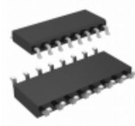
MAX4605CSE+ Maxim Integrated IC SWITCH QUAD SPST 16SOIC
