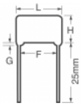
ECQ-P1H682GZ3 Panasonic Electronic Components CAP FILM 6800PF 2% 50VDC RADIAL
