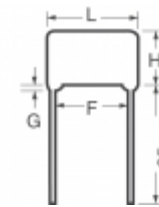
ECQ-P1H821JZ3 Panasonic Electronic Components CAP FILM 820PF 5% 50VDC RADIAL
