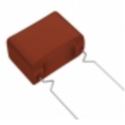
ECW-F2685HAQ Panasonic Electronic Components CAP FILM 6.8UF 3% 250VDC RADIAL
