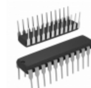
AT28C16E-20PC Microchip Technology IC EEPROM 16KBIT 200NS 24DIP
