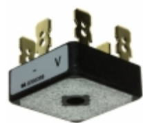
VS-36MT120 Vishay Semiconductor Diodes Division RECT BRIDGE 3-PHA 1200V 35A D-63
