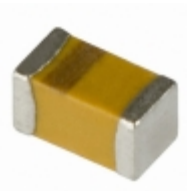
TLCL226M006RTA AVX Corporation CAP TANT 22UF 6.3V 20% 0603
