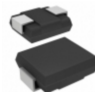
ERZ-VF2M431 Panasonic Electronic Components VARISTOR 430V 300A 2SMD JLEAD
