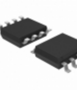
24FC512-I/SN Microchip Technology IC EEPROM 512KBIT 1MHZ 8SOIC
