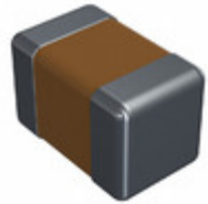
CDR01BX102BKMRAB Electro-Films (EFI) / Vishay CAP CER 1000PF 100V BX 0805
