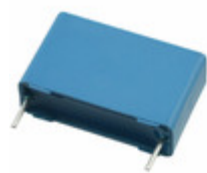
B32923C3474M189 EPCOS (TDK) CAP FILM 0.47UF 20% 305VAC RAD
