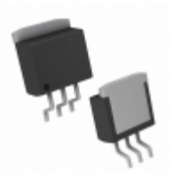
MIC39300-2.5BU TR Microchip Technology IC REG LDO 2.5V 3A TO263-3
