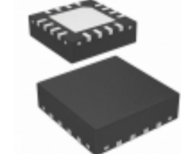
IXZ-2510 InvenSense MEMS GYROSCOPE 2-AXIS 16QFN
