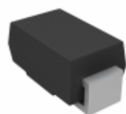
SMAJ7.5-E3/5A Vishay Semiconductor Diodes Division TVS DIODE 7.5VWM 14.3VC SMA
