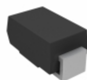
SMAJ7.5-E3/61 Vishay Semiconductor Diodes Division TVS DIODE 7.5VWM 14.3VC SMA
