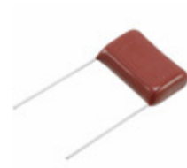
ECQ-E6394JFW Panasonic Electronic Components CAP FILM 0.39UF 5% 630VDC RADIAL
