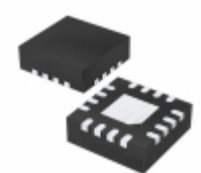
MCP4261-502E/ML Microchip Technology IC POT DGTL DUAL 5K SPI 16QFN
