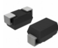
SMAJ20CA Bourns Inc. TVS DIODE 20VWM 32.4VC DO214AC
