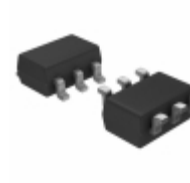
MIC5321-MMYD6-TR Microchip Technology IC REG LDO 2.8V 0.15A TSOT23-6
